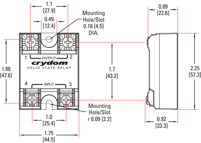
Screw Termination
