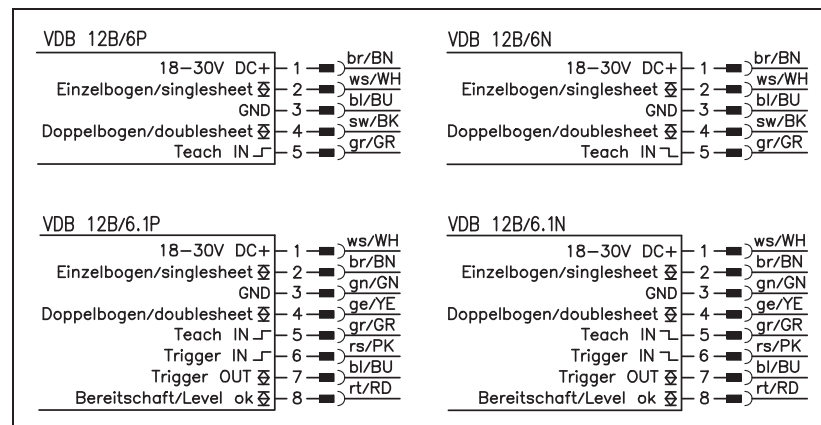
Figure 6.1: Connection diagrams VDB 12 B...
